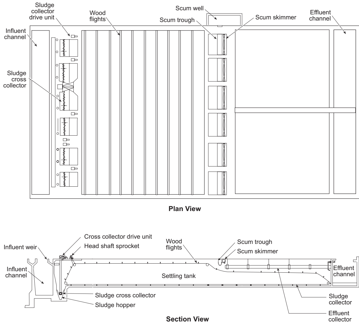
Figure T2-2. Typical Rectangular Primary Settling Tank
