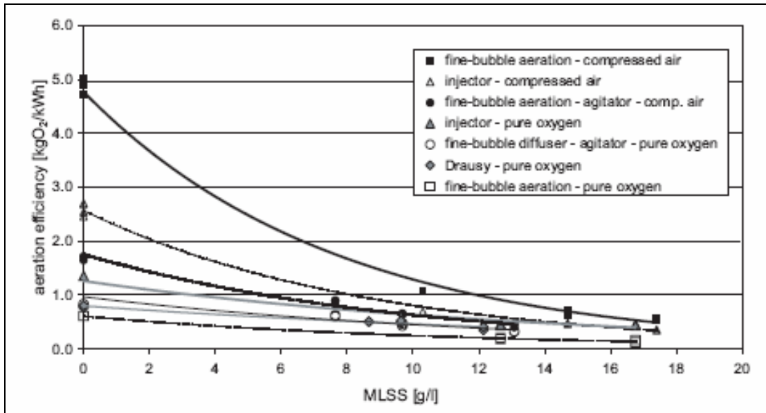
Figure T6- 1 Aeration Efficiency versus MLSS
