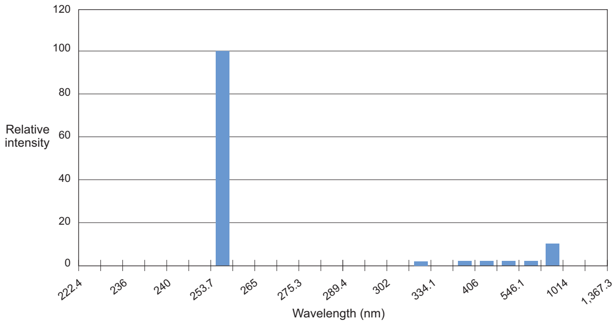
Figure T5-1. Relative Intensity of the Wavelengths Produced by the Low-Pressure Mercury Lamp
