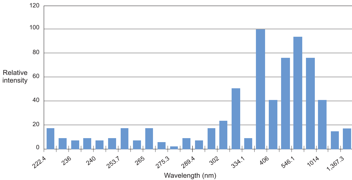
Figure T5-2. Relative Intensity of the Wavelengths Produced by the Medium-Pressure Mercury Lamp
