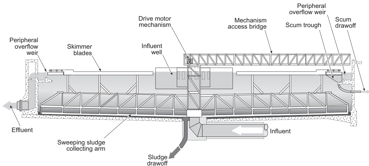
Figure T2-1. Typical Circular Primary Settling Tank
